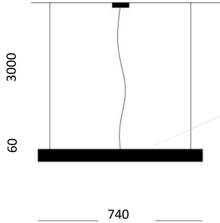
LED Driver
